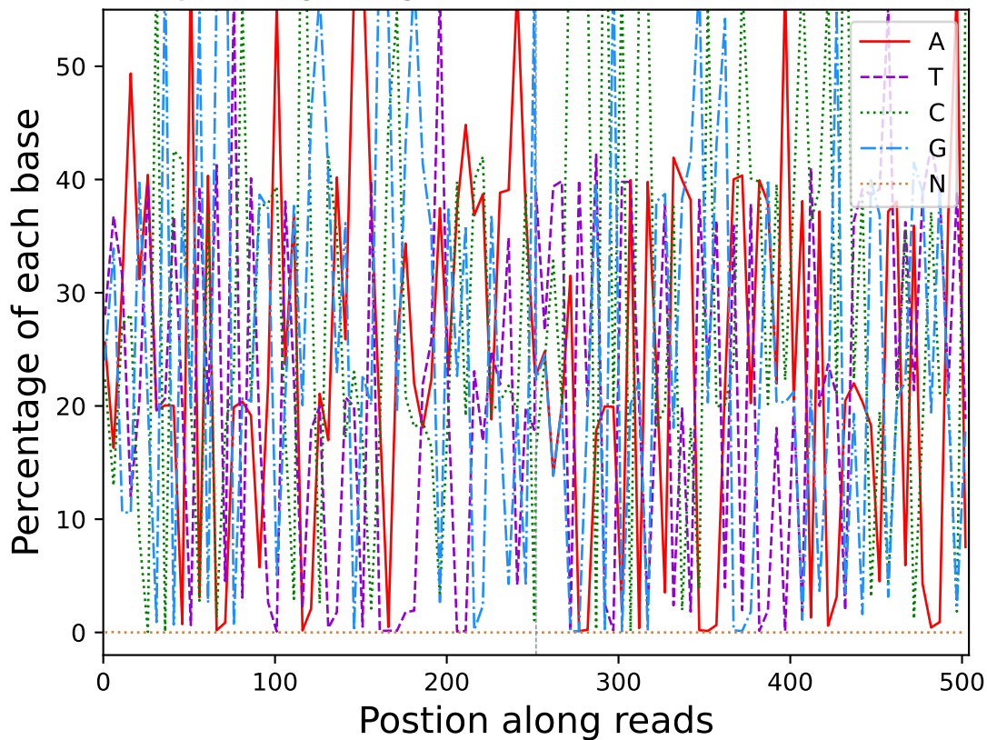
Base percentage along reads (R10219)
